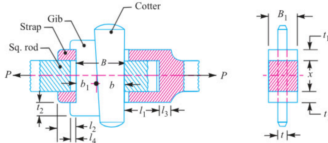
Fig. 12.13. Gib and cotter joint for square rods.
